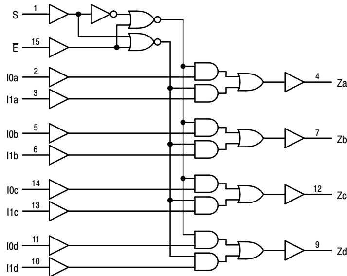
Figure 1. Logic Diagram
