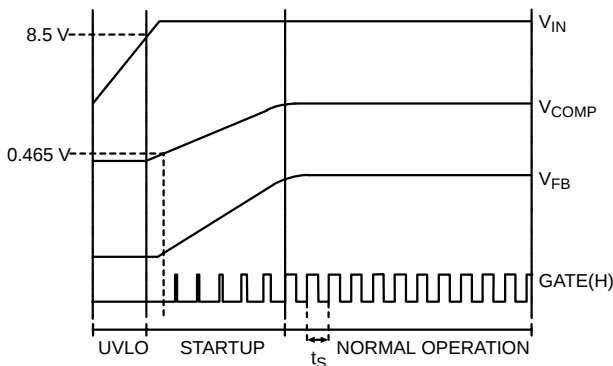
Figure 21. Idealized Waveforms
