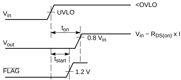
Figure 3. Start Up Sequence
