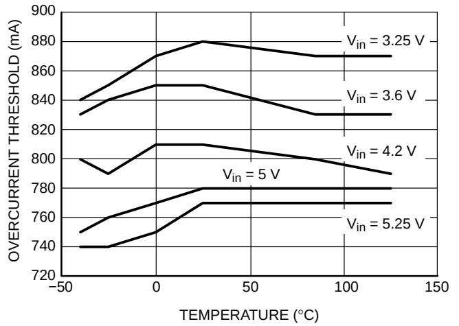
Figure 18. Overcurrent Protection Threshold vs. Temperature
