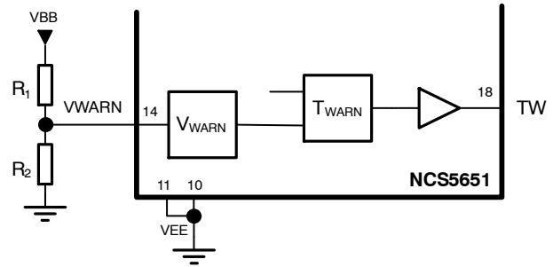
Figure 12. Setting the Thermal Warning Limit by Applying the Corresponding Threshold Voltage to Pin 14 (V WARN )
