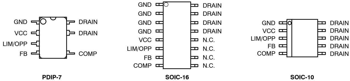
Figure 1. Pin Connections
