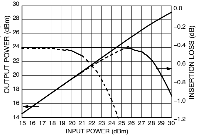
Figure 8. Output power, Insertion Loss vs Input Power Freq = 6.0 GHz, IN-OUT2 ON
