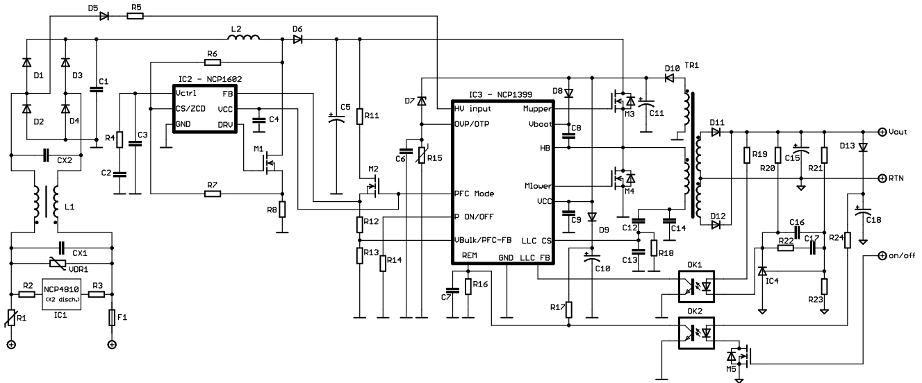
Figure 3. Typical Application Example with PFC Stage (Active ON off-mode)
