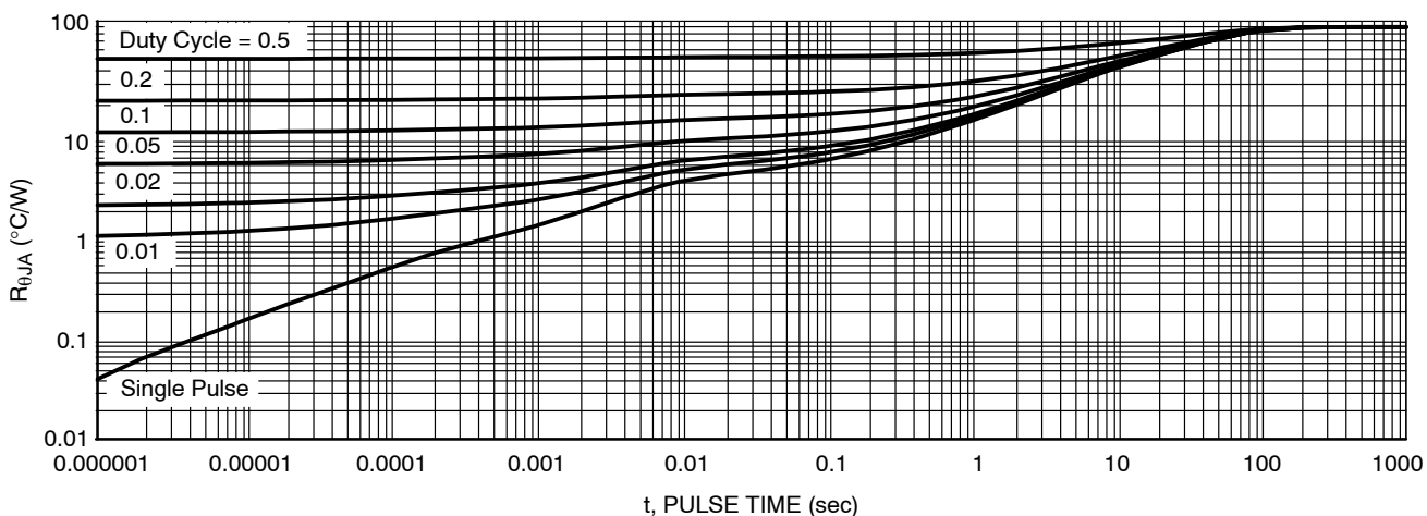
Figure 5. Thermal Response
