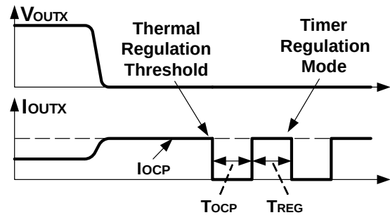
Figure 6. Short Circuit
