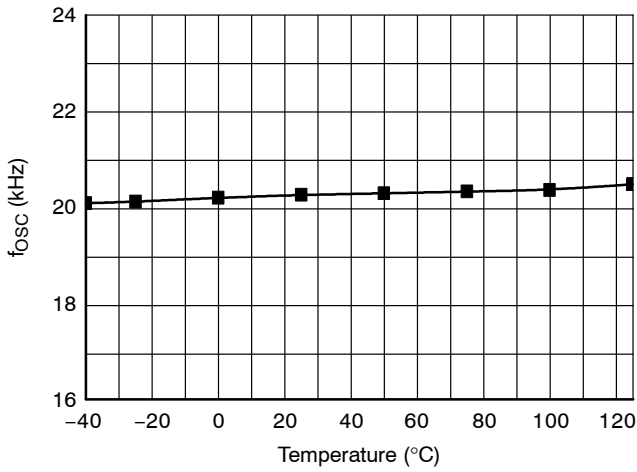
Figure 18. f OSC vs. Temperature (R t = 87 kΩ)
