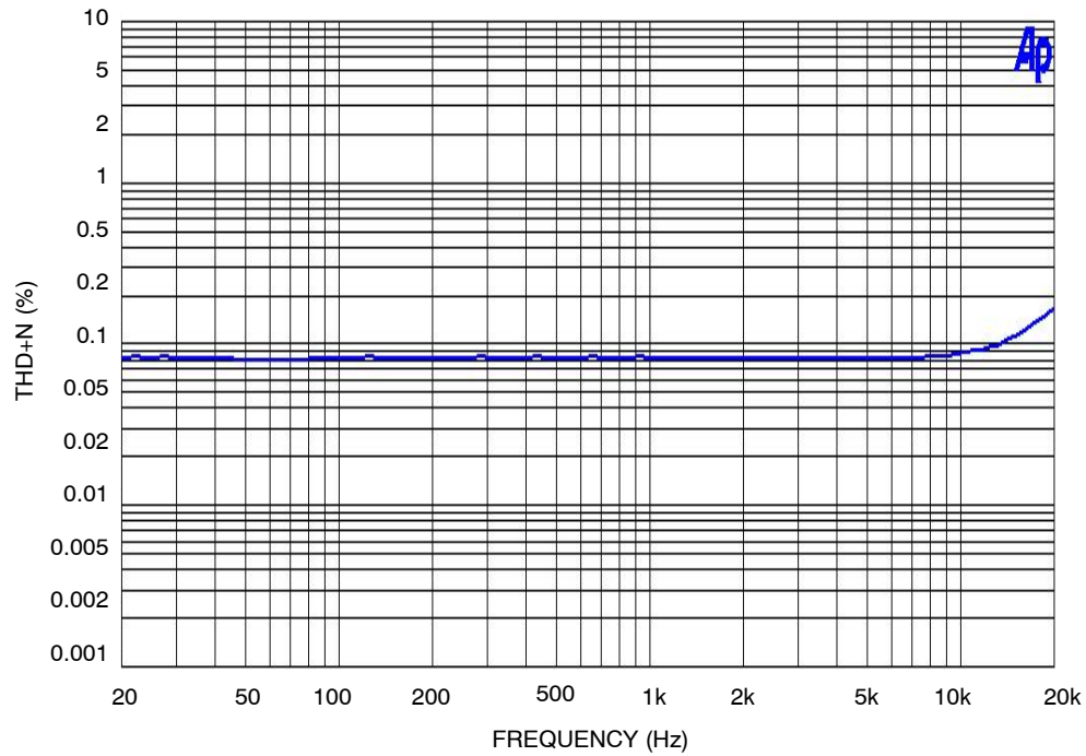
Figure 9. THD+N
