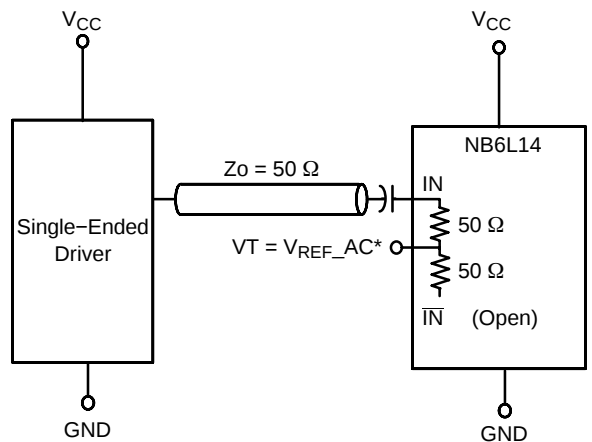
Figure 19. Capacitor-Coupled Single-Ended Interface (VT Connected to V REFAC )
