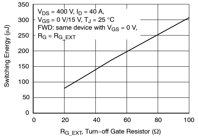
Figure 22. Clamped Inductive Switching Turn-off Energy vs. R_{G\_EXT} , Turn-off Gate Resistor
