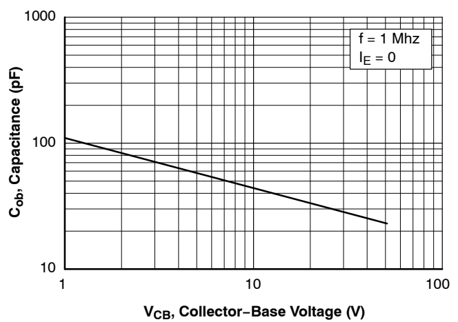
Figure 4. Collector-Base Voltage
