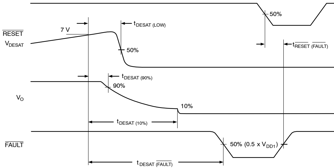
Figure 56. Definitions for Fault Reset Input ( \overline{RESET} ), Desaturation Voltage Input ( V_{DESAT} ), Output Voltage ( V_O ), and Fault Output ( \overline{FAULT} ) Timing Waveforms
