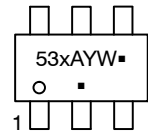
TSOP-6 CASE 318G STYLE 13
