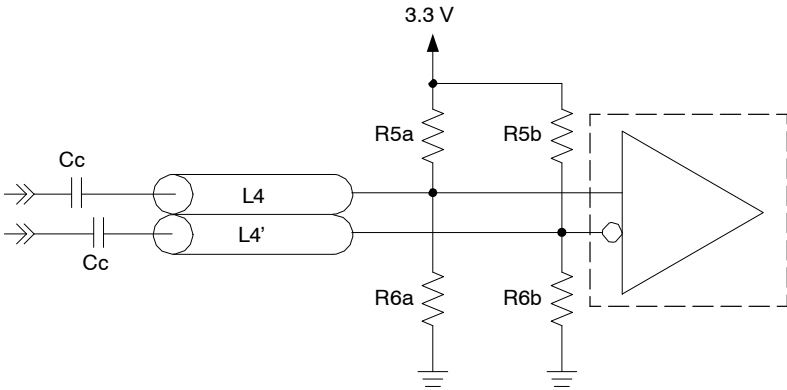
Figure 9. Cable-Connected AC Coupled Application
