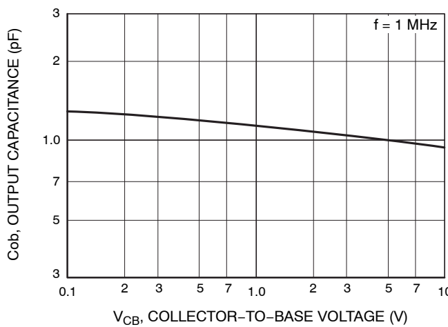
Figure 5. C_{ob} - V_{CB}
