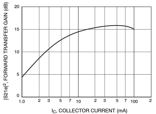
Figure 6. |S_{21e}|^2 - I_C
