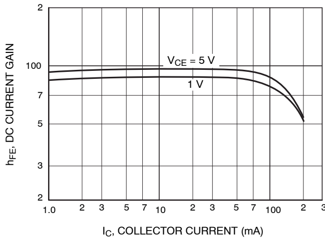
Figure 3. h_{FE} - I_C
