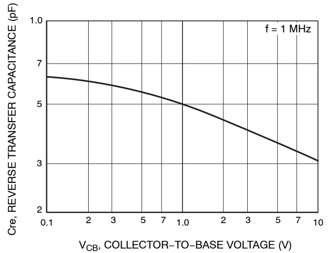
Figure 4. C_{re} - V_{CB}
