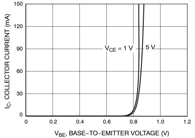
Figure 2. I_C - V_{BE}
