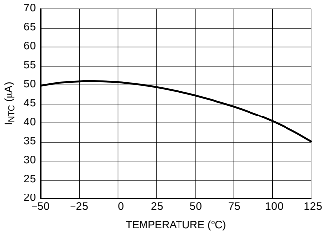
Figure 21. Current I_{NTC} Sourced from the Latch Pin, Allowing Direct NTC Connection
