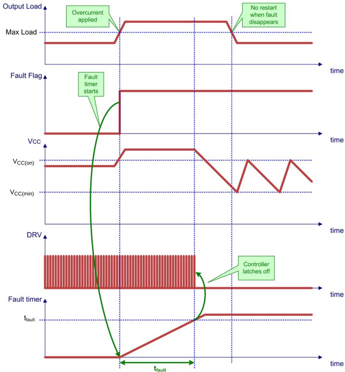
Figure 71. Latched Timer-Based Overcurrent Protection (Option G)
