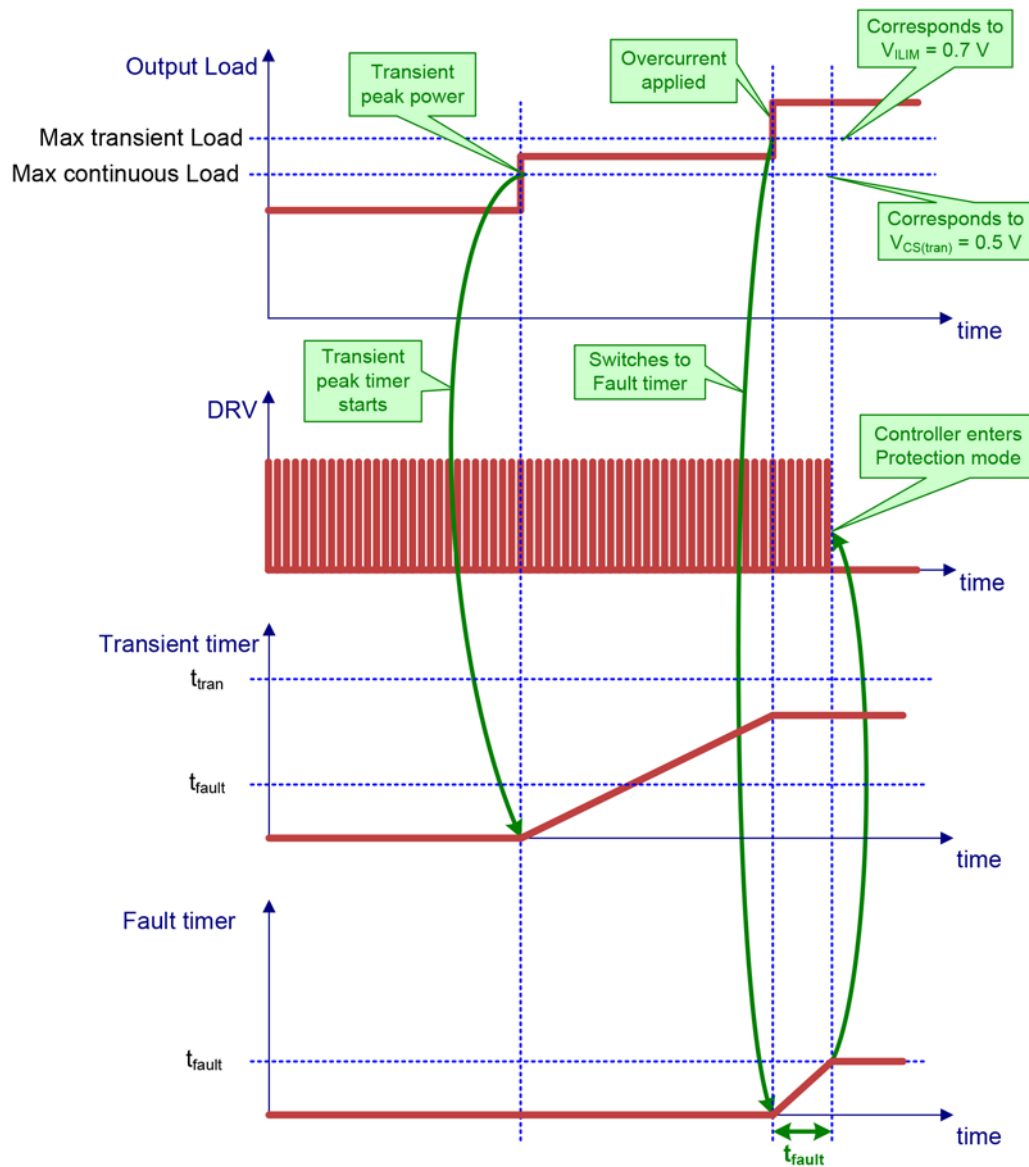
Figure 73. Transient Peak Power Followed by Overload
