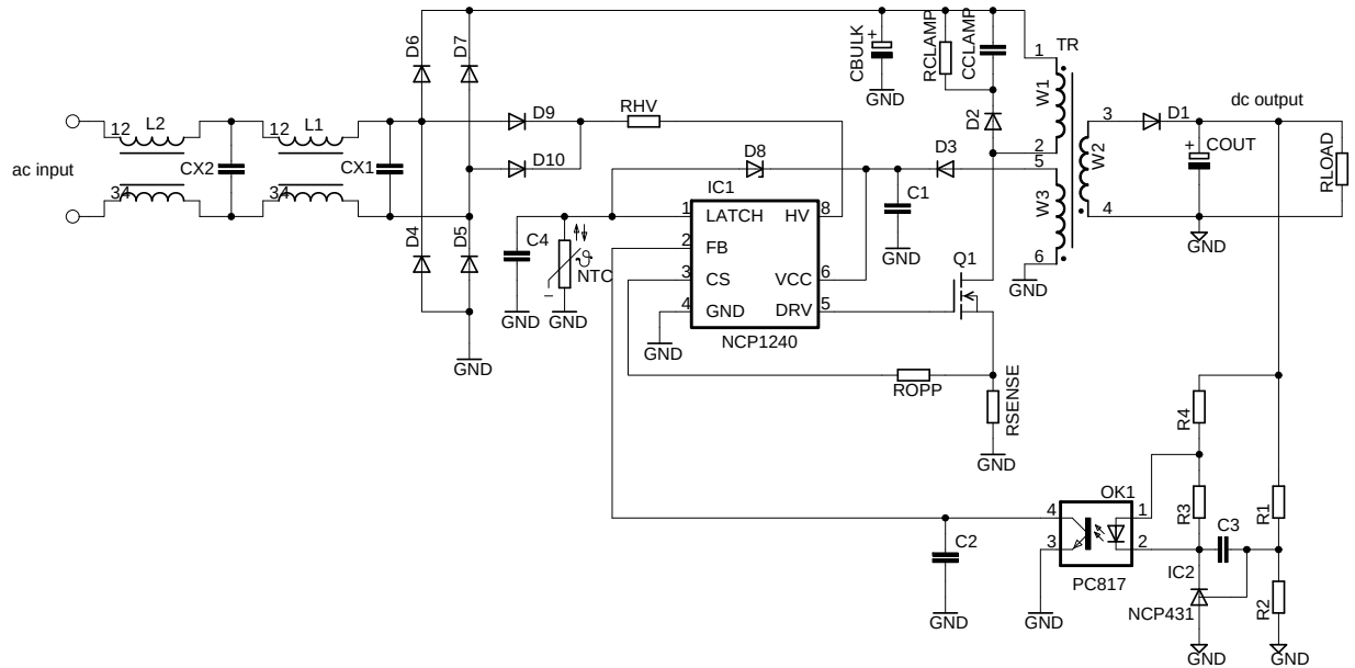
Figure 1. Flyback Converter Application Using the NCP1240G
