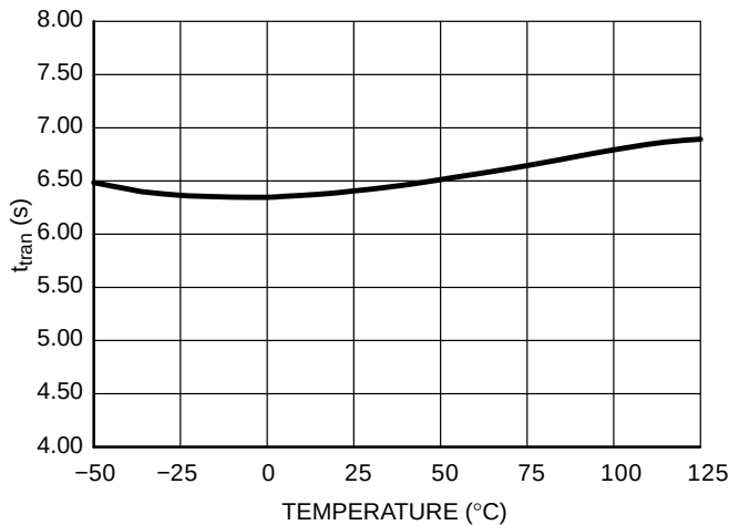
Figure 43. Transient Peak Power Timer Duration t_{tran}
