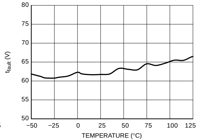
Figure 42. Fault Timer Duration t_{fault}
