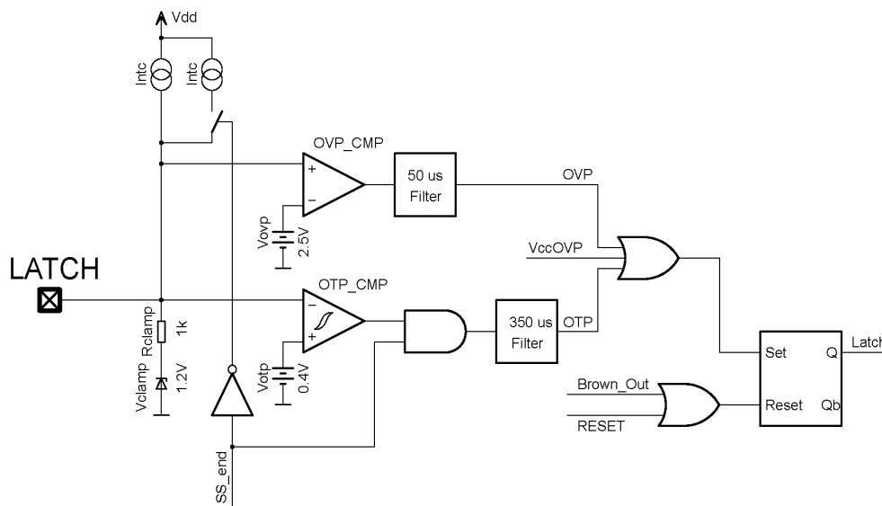
Figure 74. Latch Detection Schematic
