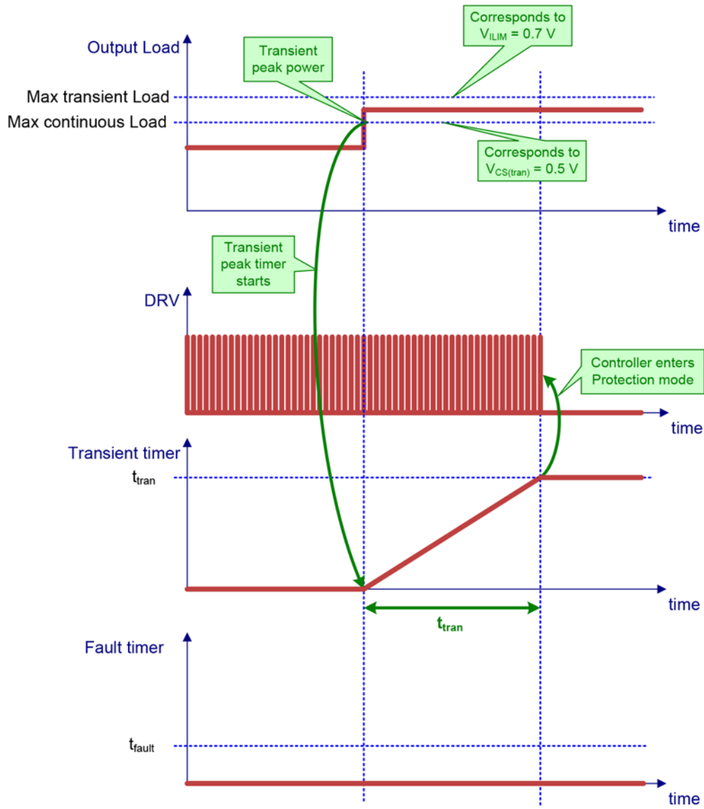
Figure 72. Too Long Transient Peak Power Delivery
