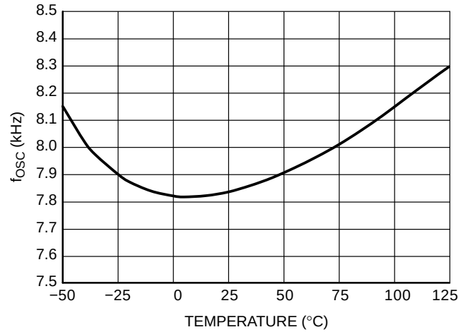
Figure 24. Maximum ON Time t_{ONmax} for the 65 kHz Version
