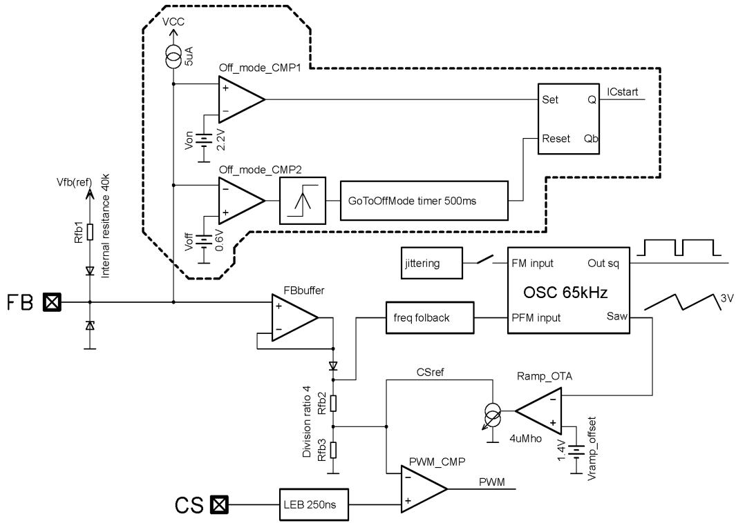
Figure 64. Slope Compensation Block Diagram
