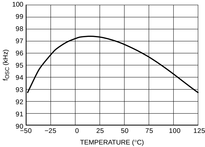
Figure 23. Oscillator f_{osc} for the 65 kHz Version
