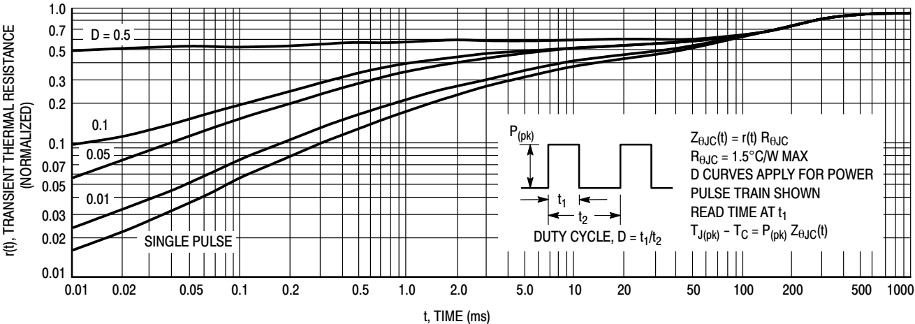
Figure 9. Thermal Response
