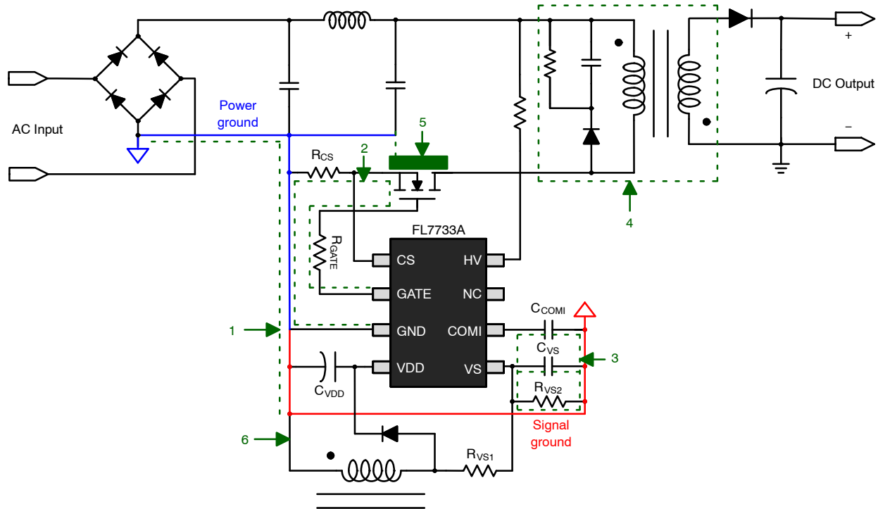
Figure 26. Layout Example
