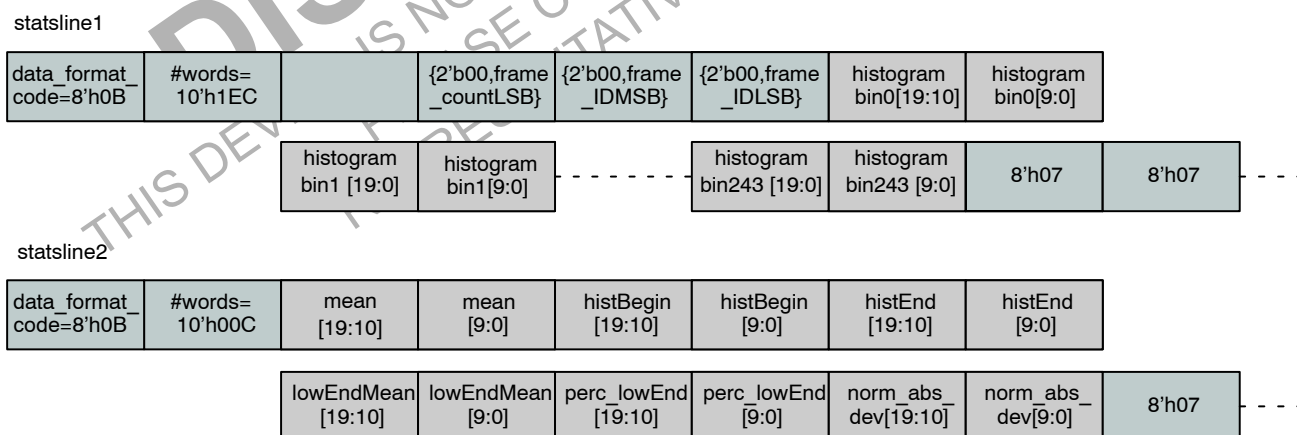
Figure 17. Format of Embedded Statistics Output within a Frame
