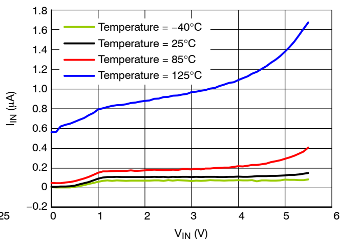
Figure 9. Standby Current ( \mu A ) versus V_{IN} (V), V_{out} Short to GND.
