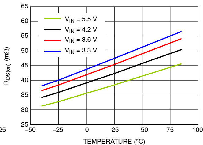
Figure 7. R_{DS(on)} ( m\Omega ) vs. Temperature ( ^{\circ}C ), I_{load} 2 A
