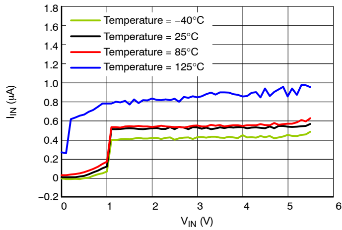
Figure 10. Quiescent Current ( \mu A ) versus V_{IN} (V), No load.
