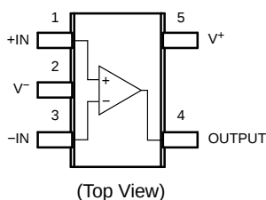
SC70-5
