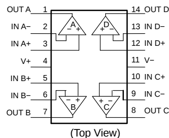
TSSOP-14
