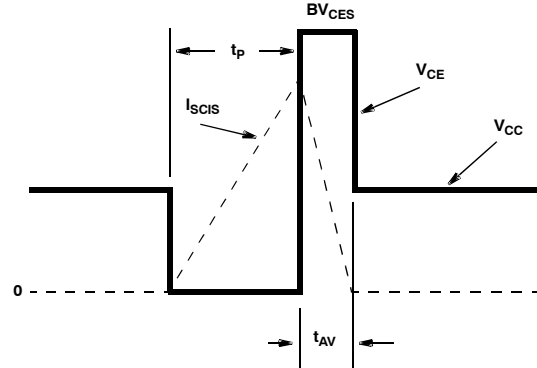
Figure 21. Energy Waveforms
