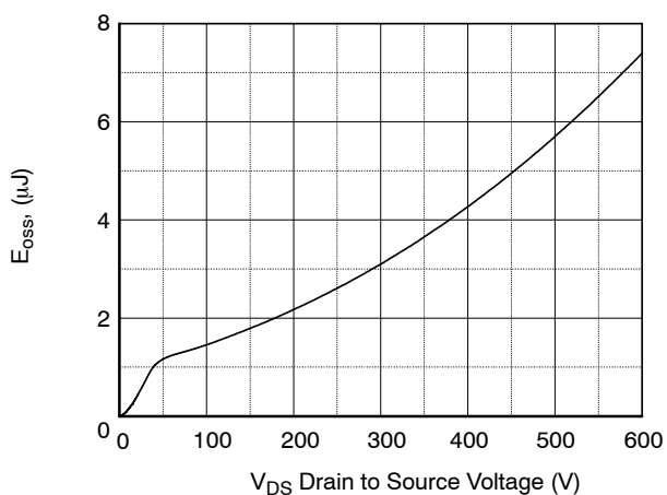
Figure 12. E_{OSS} vs. Drain to Source Voltage
