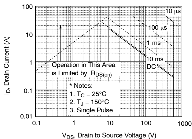
Figure 9. Maximum Safe Operating Area for FCP260N60E
