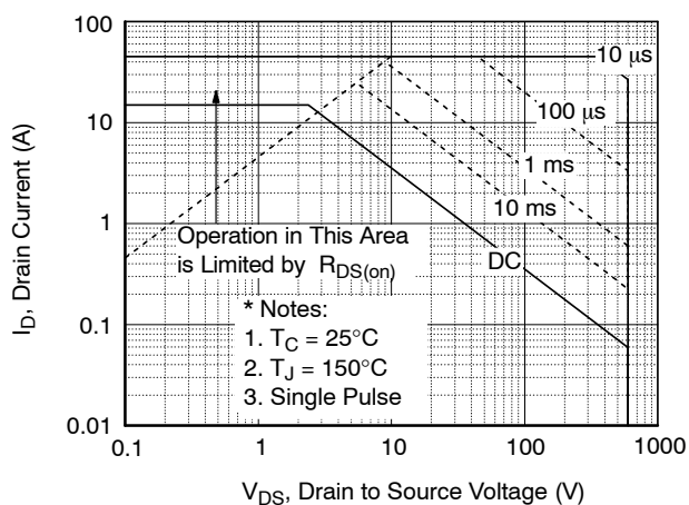
Figure 10. Maximum Safe Operating Area for FCPF260N60E
