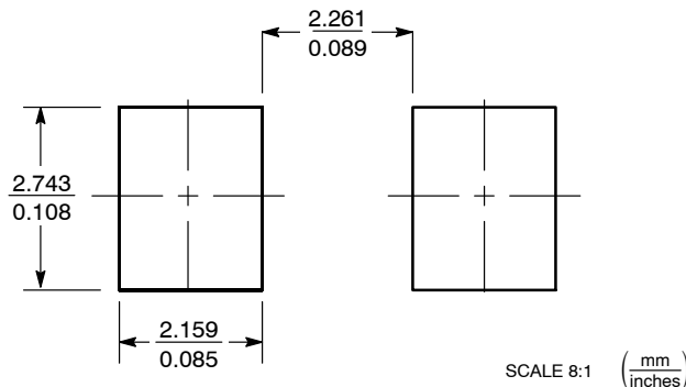
SOLDERING FOOTPRINT*
