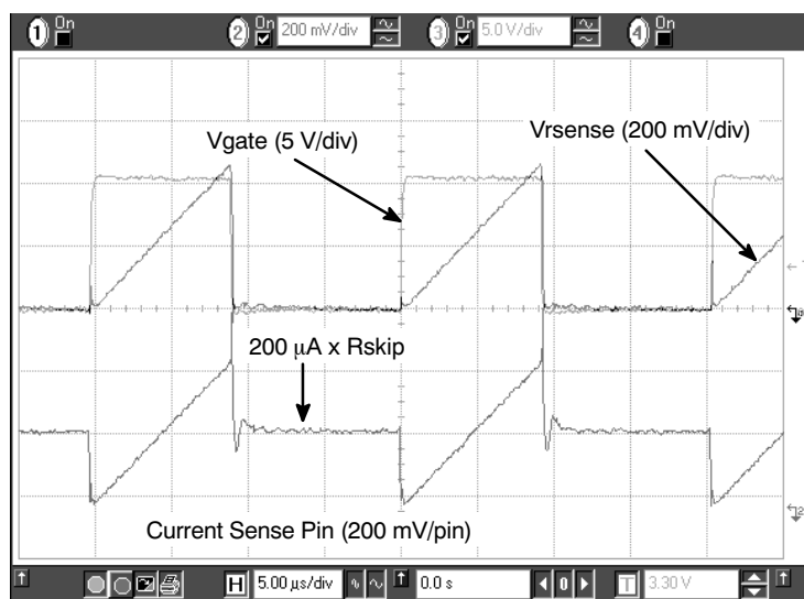
Figure 26. This picture explains how the 200\text{ }\mu\text{A} internal offset current creates the skip cycle level.
