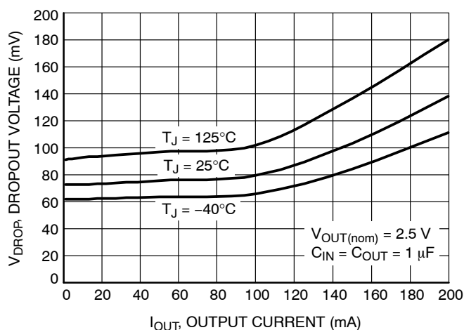
Figure 19. Dropout Voltage vs. Output Current, V OUT = 2.5 V
