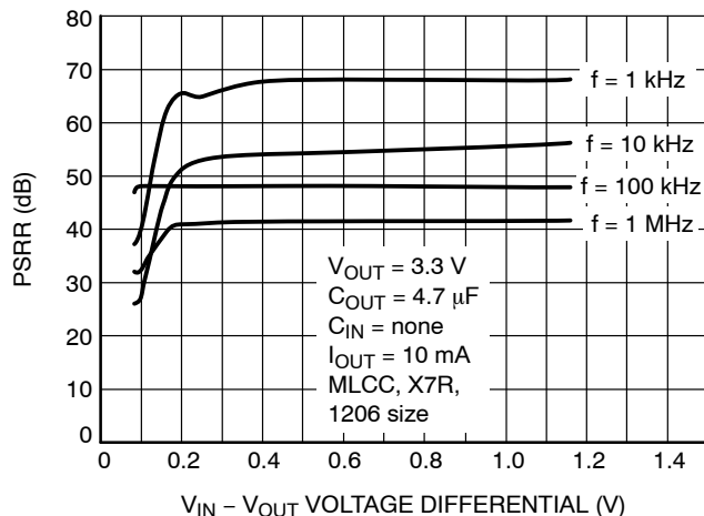
Figure 15. PSRR vs. Voltage Differential, C OUT = 4.7 μF, I OUT = 10 mA
