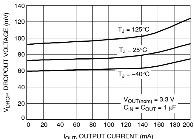
Figure 18. Dropout Voltage vs. Output Current, V OUT = 3.3 V
