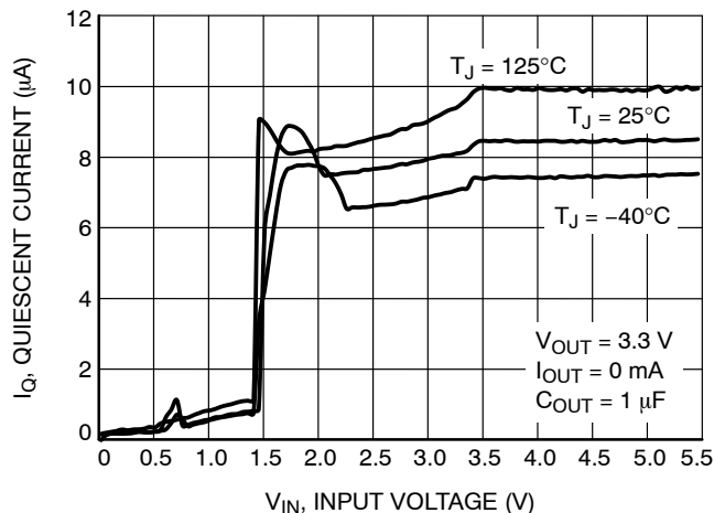
Figure 16. Quiescent Current vs. Input Voltage, V OUT = 3.3 V
