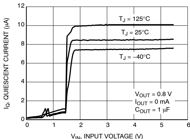
Figure 17. Quiescent Current vs. Input Voltage, V OUT = 0.8 V
