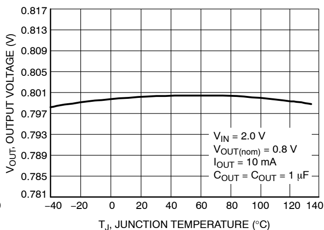
Figure 20. Output Voltage vs. Temperature, V OUT = 0.8 V
