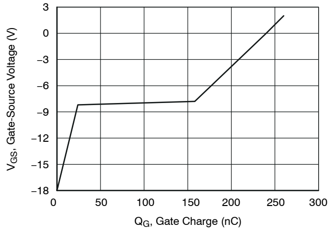
Figure 16. Typical Gate Charge at V_{DS} = 400 V and I_D = 60 A
