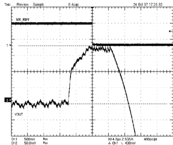
Figure 22. VR11.1, 1.6 V OVP Event
