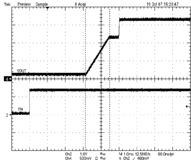
Figure 9. VR11.1 Startup
