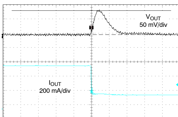
Figure 24. 600 mA to 200 mA Load Transient ( V_{IN} = 3.6\text{ V} , V_{OUT} = 1.2\text{ V} , T_A = 25^\circ\text{C} )
