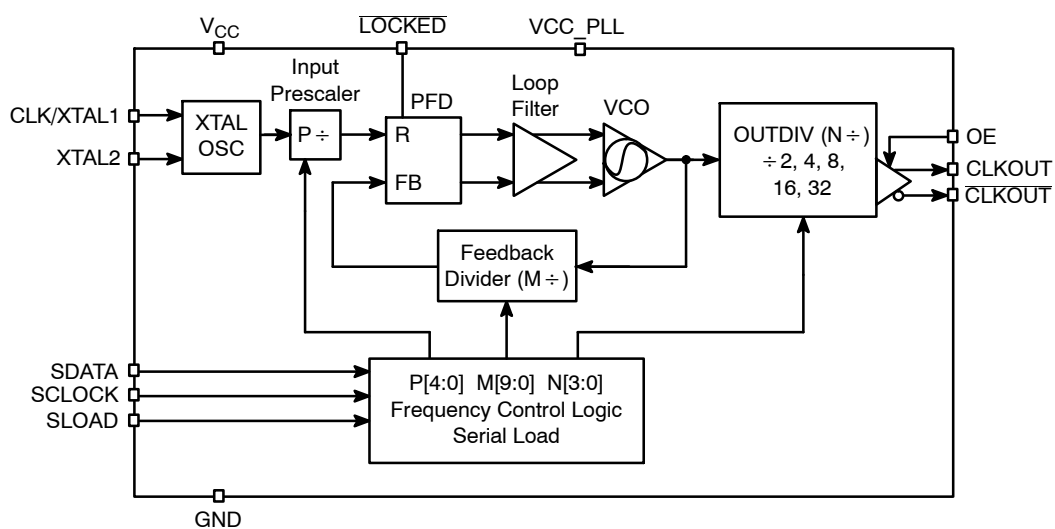
Figure 2. Block Diagram
