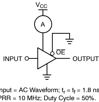
Figure 5. I_{CCD} Test Circuit
