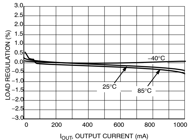
Figure 29. Load Regulation vs. Output Current ( V_{IN} = 5.0 \text{ V} , V_{OUT} = 3.9 \text{ V} )
