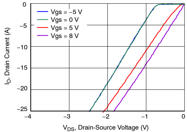
Figure 10. 3 rd Quadrant Characteristics at T_J = 25\text{ }^{\circ}\text{C}
