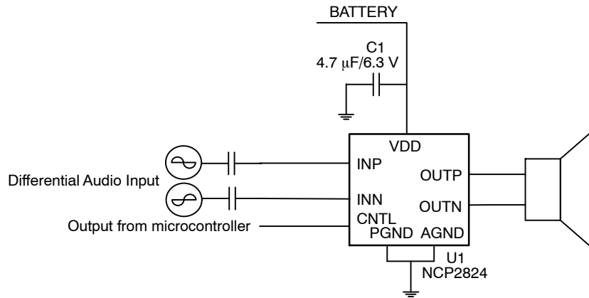
Figure 18. Differential Configuration
