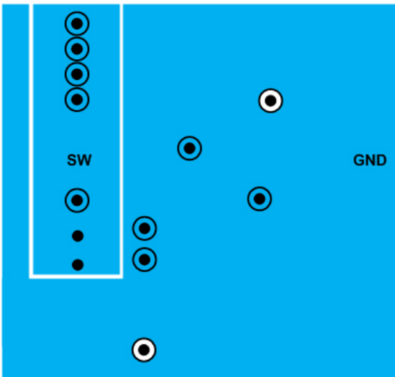
Figure 27. Mid-Layer 2
