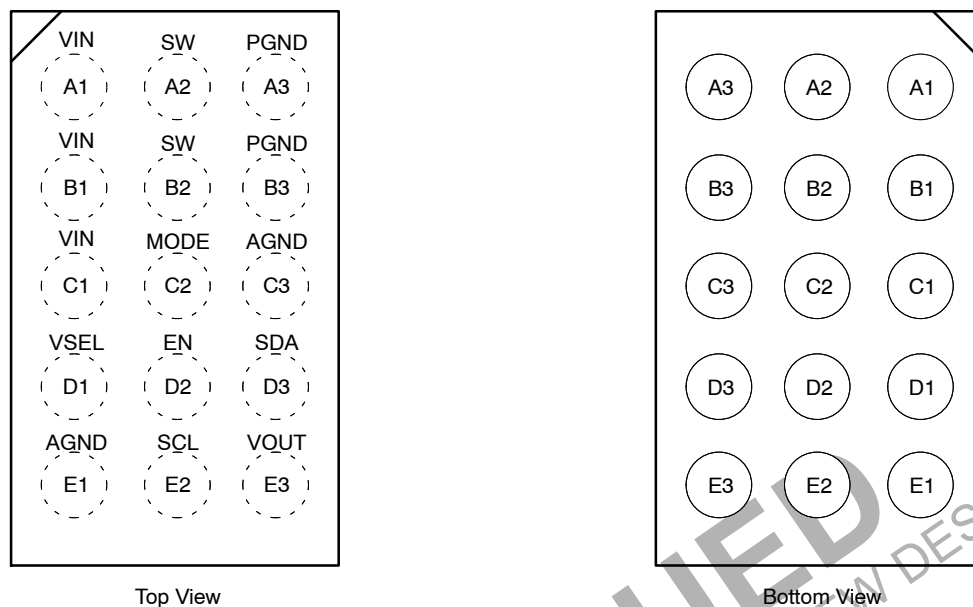
Figure 2. Pin Configuration
