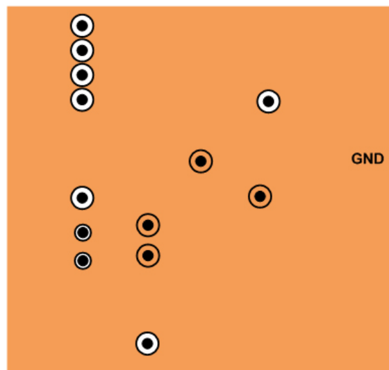
Figure 26. Mid-Layer 1
