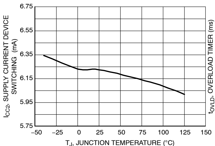
Figure 38. Supply Current Device Switching vs. Junction Temperature
