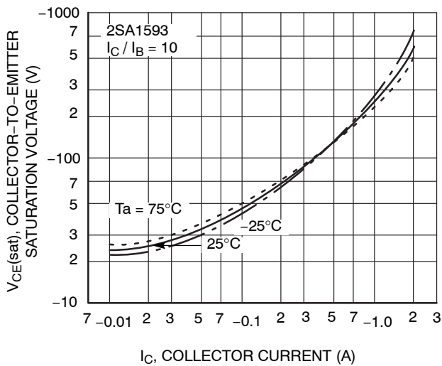
Figure 12. V_{CE(sat)} - I_C
