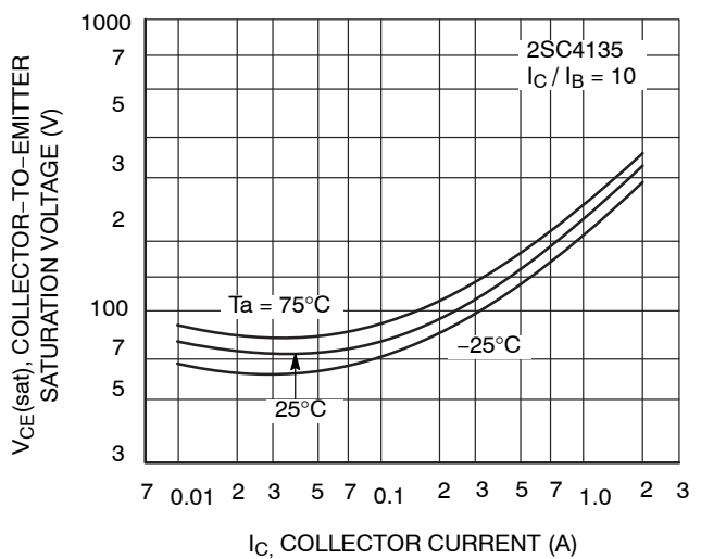
Figure 13. V_{CE(sat)} - I_C
