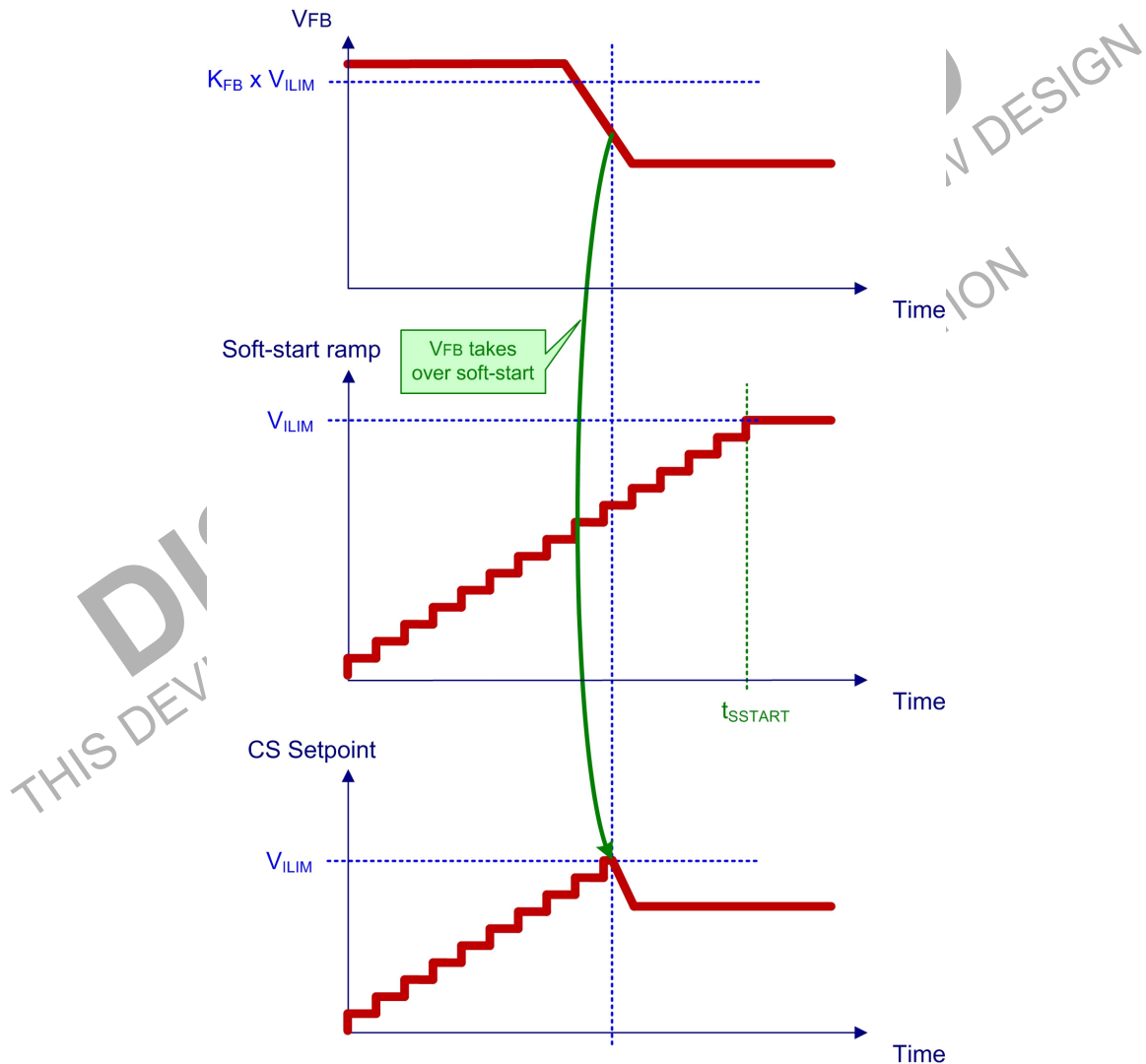
Figure 57. Soft-Start Feature
