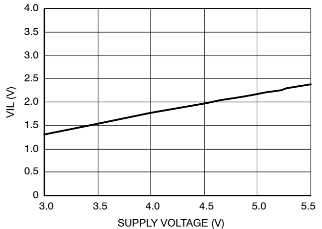
Figure 24. SDA, SCL V_{IL} vs. Supply Voltage
