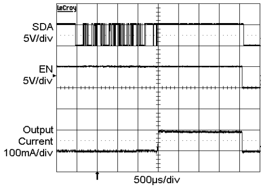
Figure 17. Enable Power Down (1x Mode)
