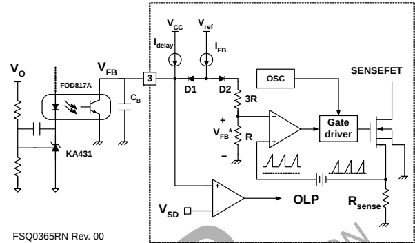
Figure 21. Pulse-Width-Modulation Circuit
