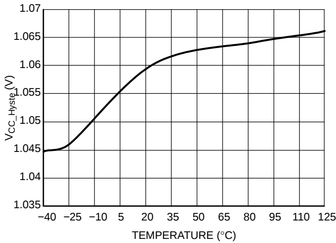
Figure 6. V_{CC} Hysteresis
