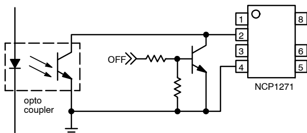
Figure 41. Non-Latchoff Shutdown
