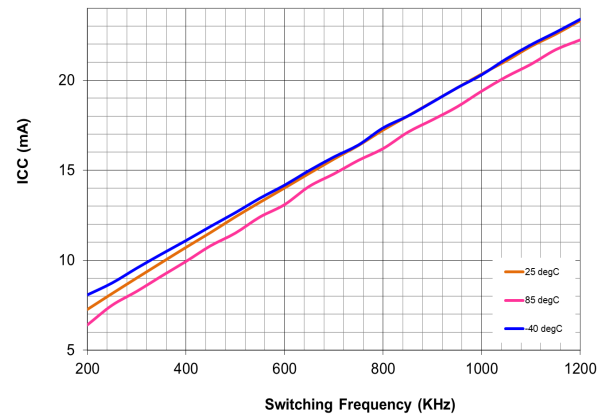
Figure 12. I_{CC} vs. Switching Frequency and Ambient Temperature
