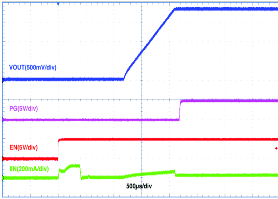
Figure 7. Start-up, No Load
