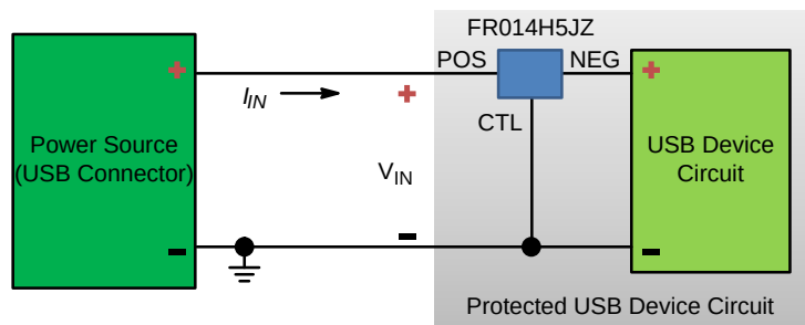
Figure 2. Typical Schematic
