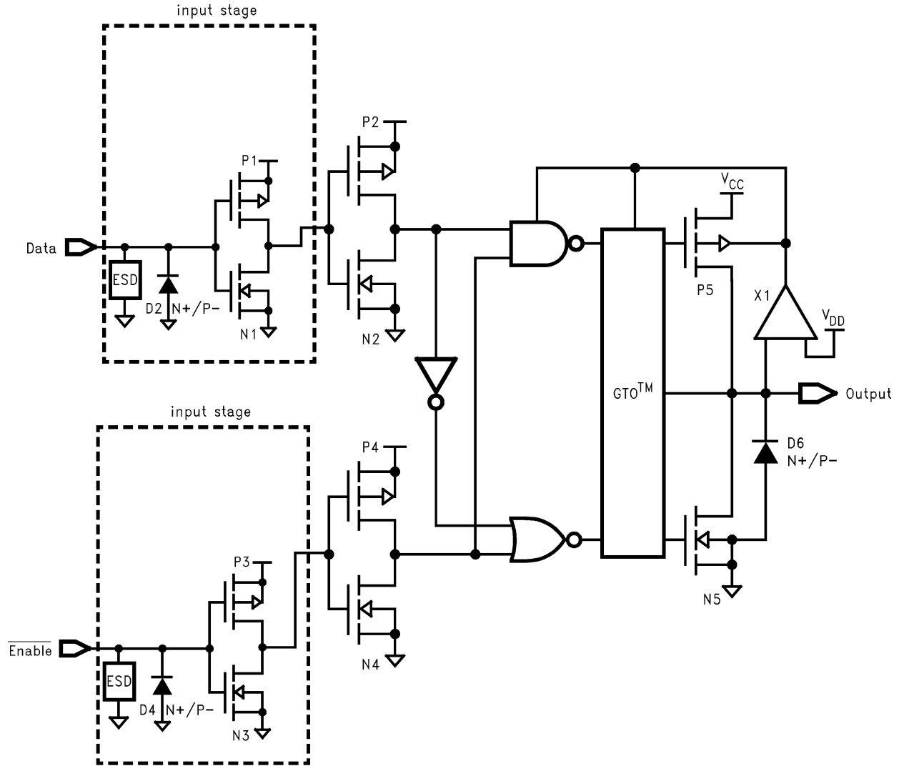
Figure 4. Schematic Diagram
