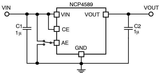
Figure 87. Typical Application Schematic
