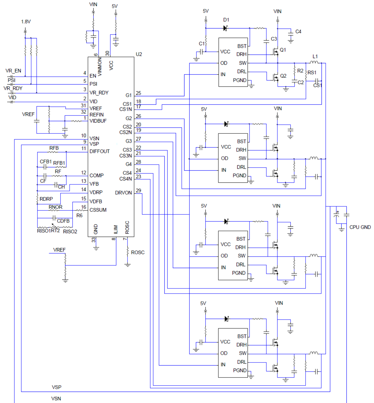
Figure 2. Typical Four Phase Application Circuit with PWM-VID Interface
